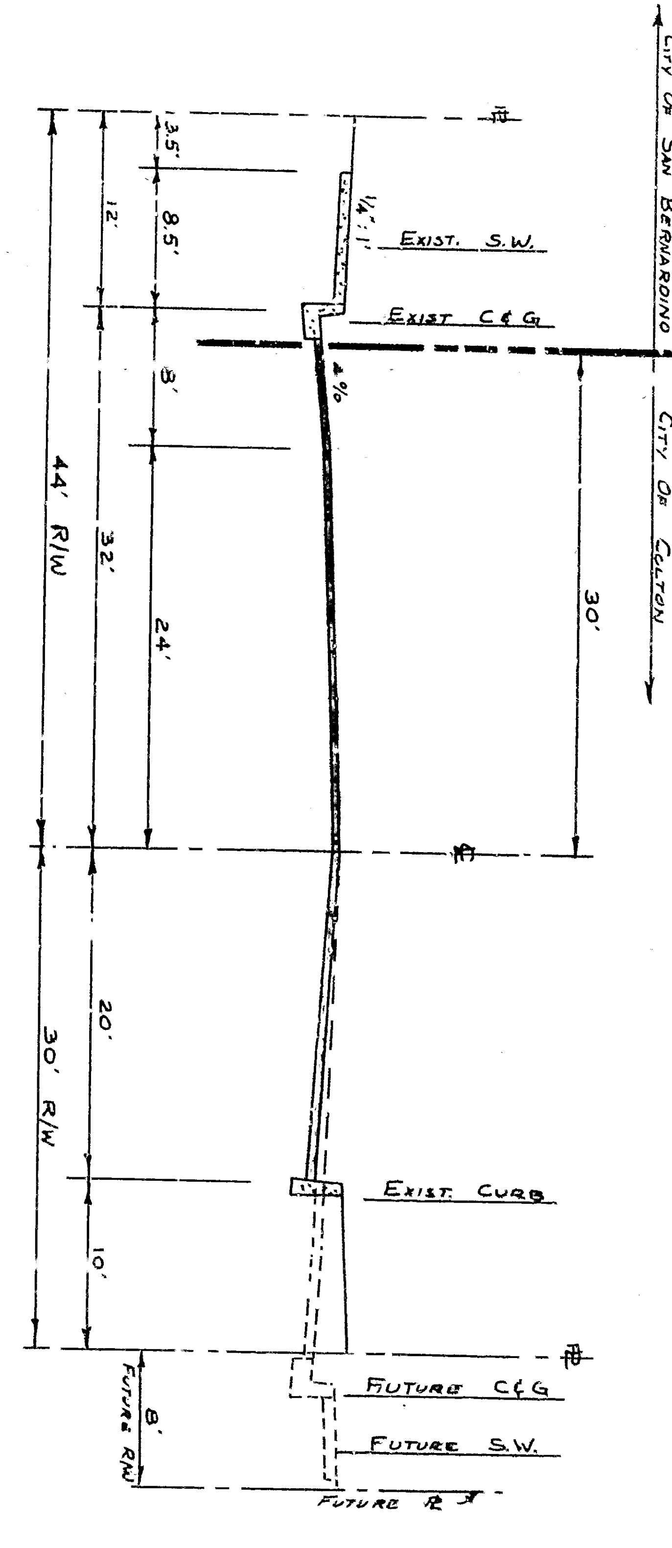
"X" SECTION STA 3+66.28 TO STA 3+94.50 (NOT A PART OF THIS CONTRACT)
